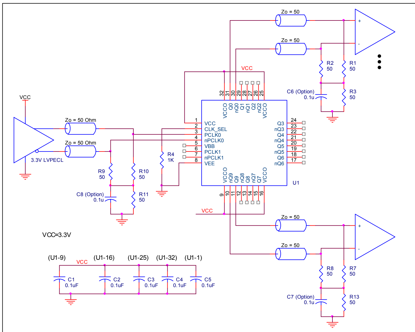
Figure 5. ICS853S111AI Example LVPECL Clock Output Buffer Schematic
