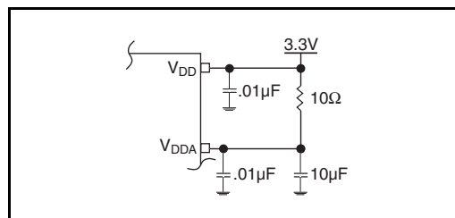
Figure 2. Power Supply Filtering
