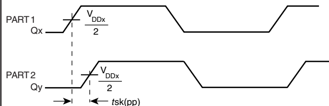
Part-to-Part Skew
