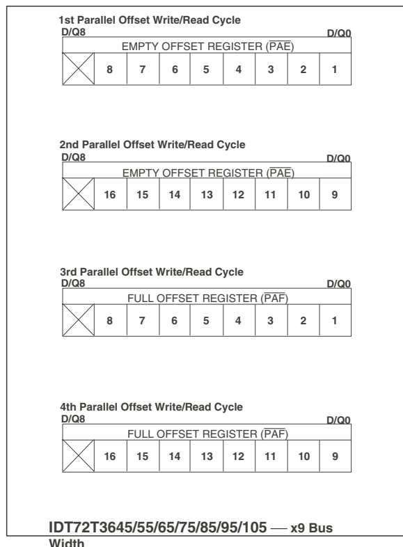
Figure 3. Programmable Flag Offset Programming Sequence (Continued)
