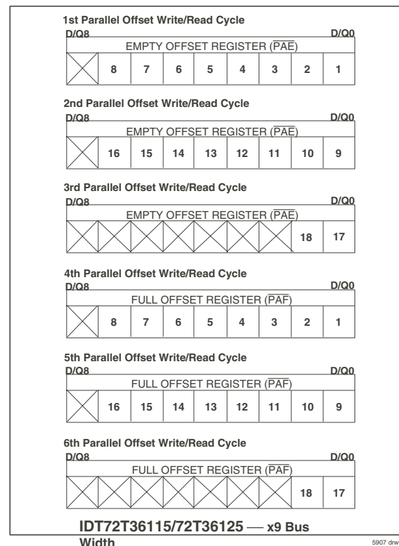
Figure 3. Programmable Flag Offset Programming Sequence (Continued)
