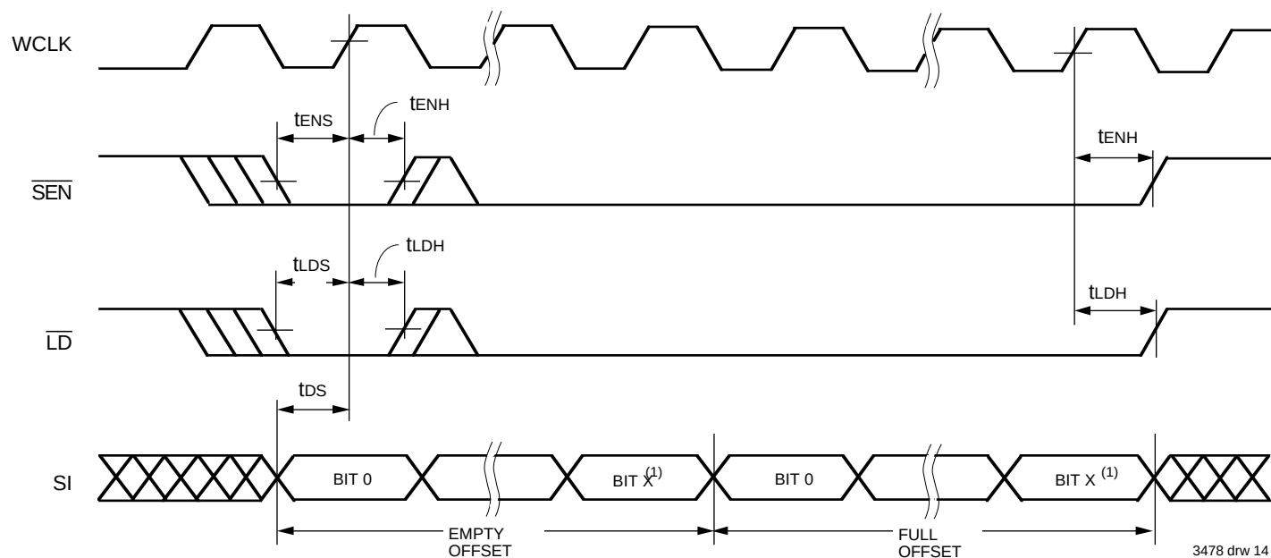
Figure 11. Serial Loading of Programmable Flag Registers (IDT Standard and FWFT modes)
