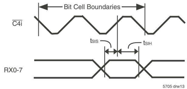
Figure 9. Serial Inputs
