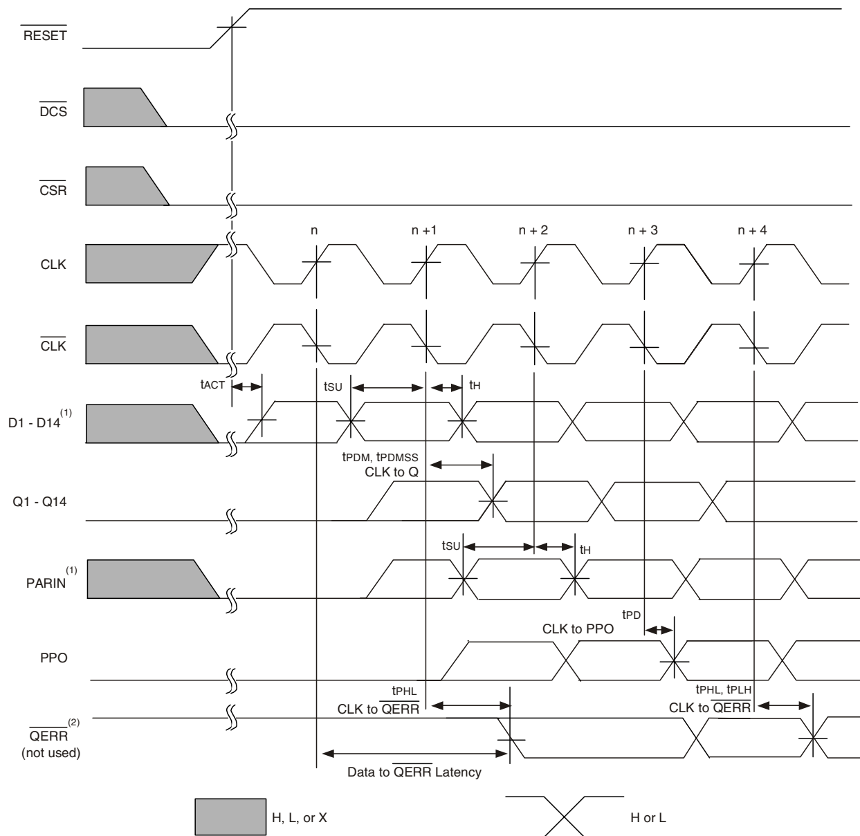
Timing Diagram for the First SSTUBF32866B (1:2 Register-A Configuration) Device Used in a Pair; \text{C0} = 0 , \text{C1} = 1 , \overline{\text{RESET}} Switches from L to H
