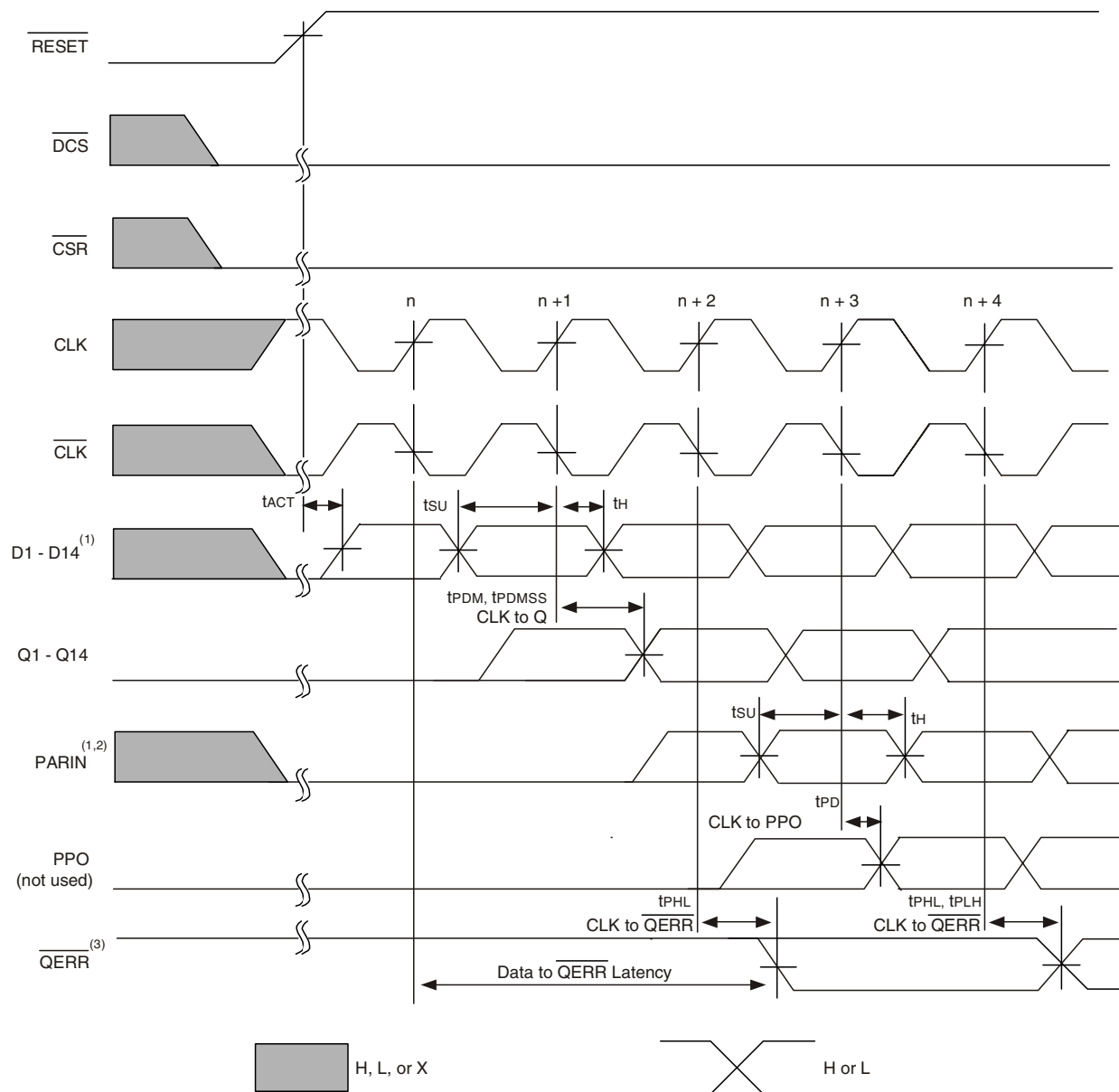
Timing Diagram for the Second SSTUBF32866B (1:2 Register-B Configuration) Device Used in a Pair; C0 = 1, C1 = 1, \overline{RESET} Switches from L to H
