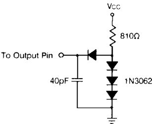
Figure 4. Output Load 1
