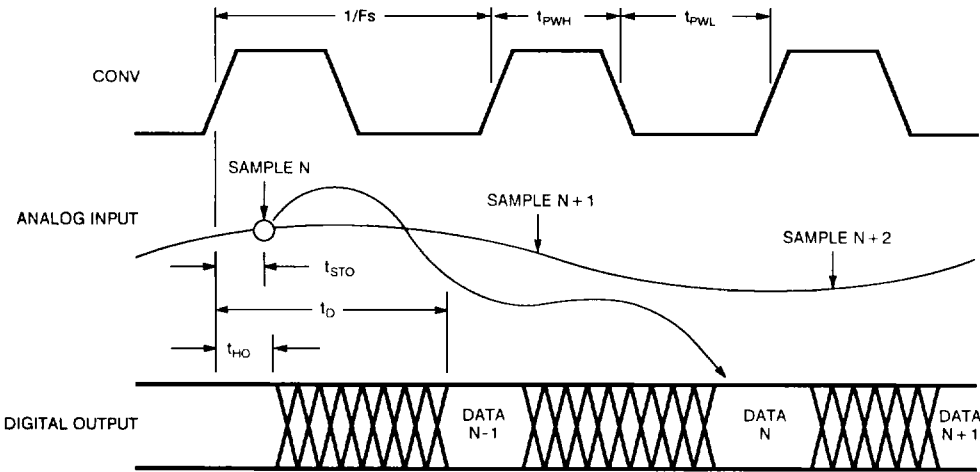
Figure 2. Timing Diagram
