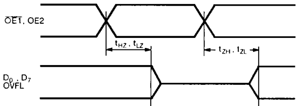
Figure 3. Output, Enable/Disable Timing
