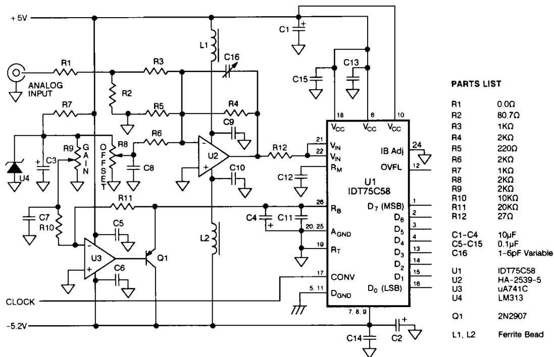
Figure 5. Application Example
