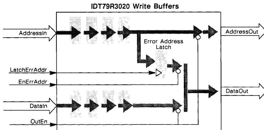
Figure 8. The Write Buffer Error Address Latch
