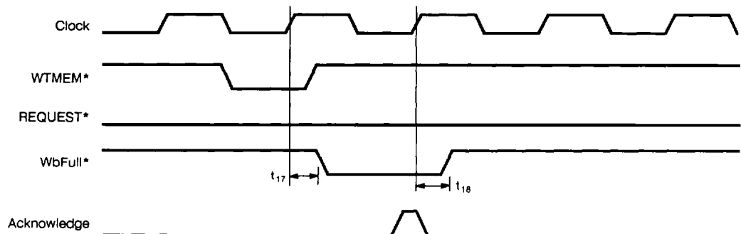
Figure 10. WBFULL* Signal Timing Specifications
