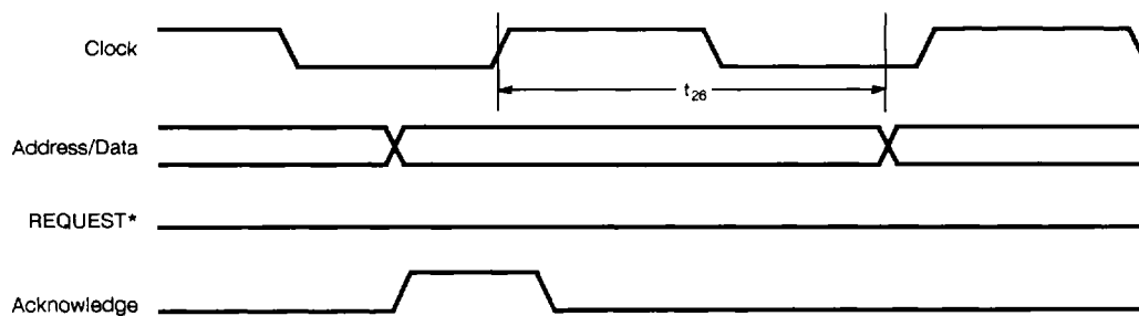
Figure 13. Address/Data Out
