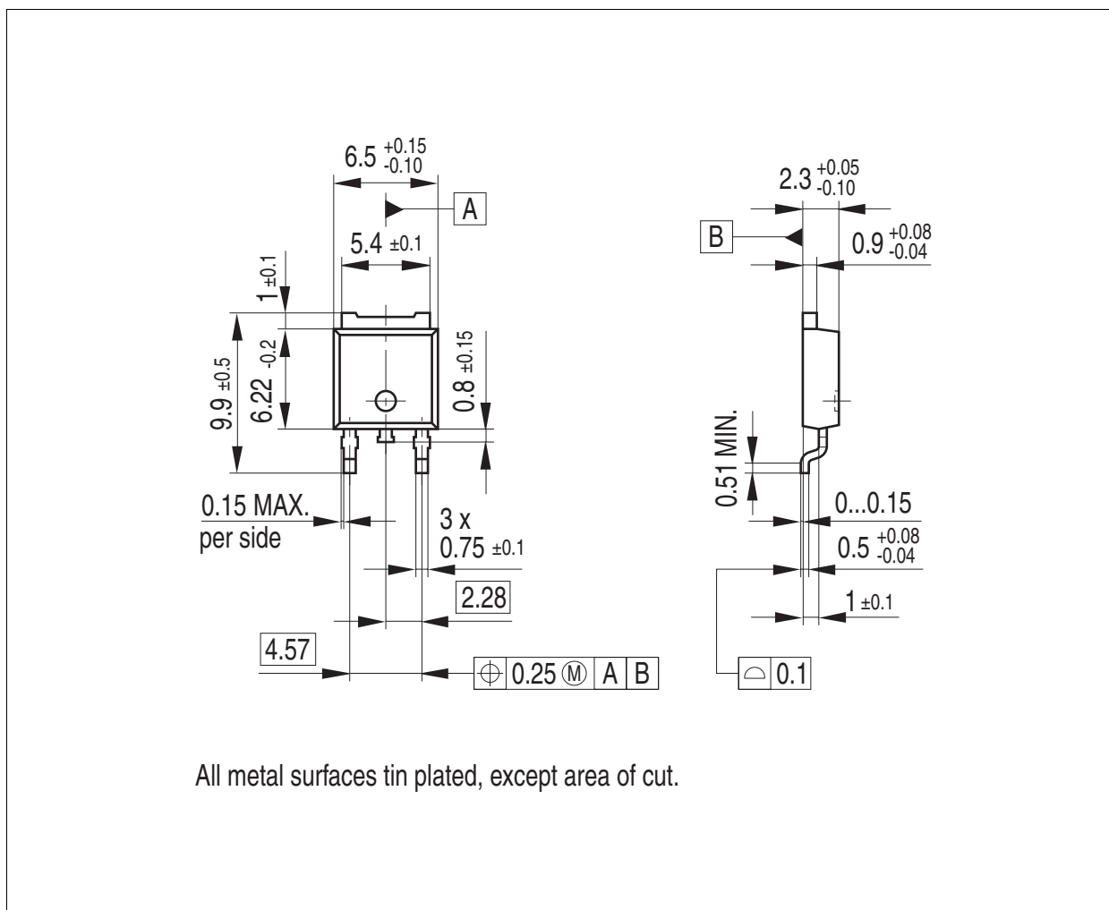
Figure 3 PG-T0252-3
