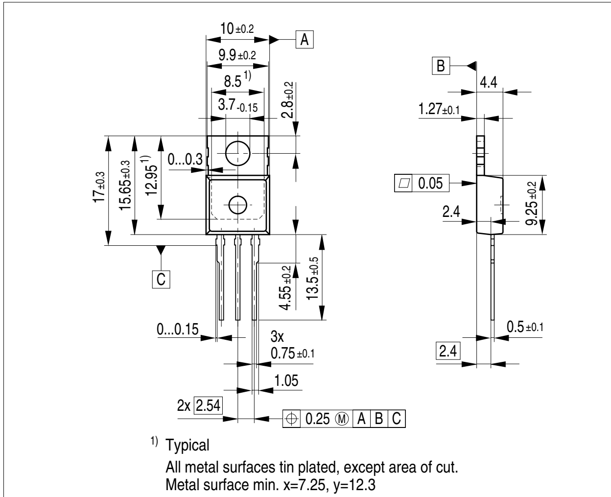
Figure 5 PG-TO220-3
