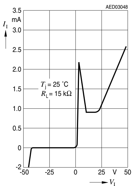
Input Current I_I versus Input Voltage V_I
