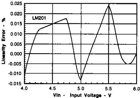
Figure 20. Linearity error vs. input voltage
