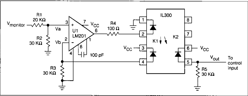
Figure 19. Transfer gain
