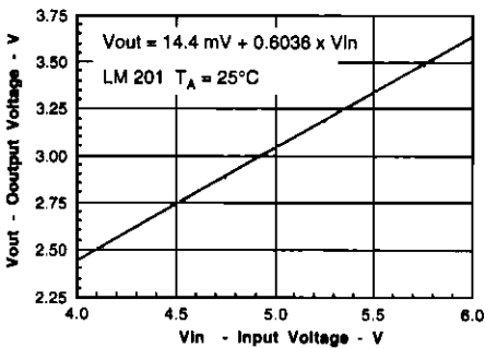
Figure 19. Transfer gain
