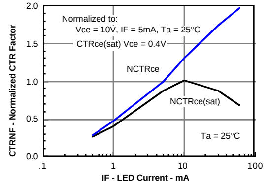
Figure 11. Normalization factor for non-saturated and saturated CTR T_A=25^\circ\text{C} versus if
