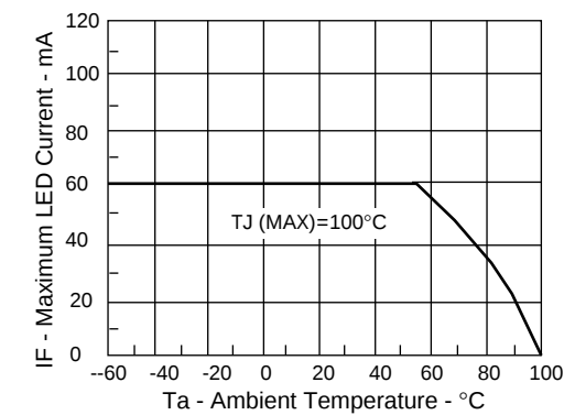
Figure 5. Maximum LED current versus ambient temperature
