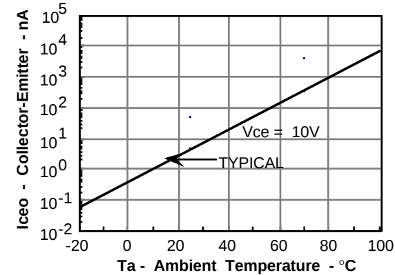
Figure 16. Collector-emitter leakage versus temperature
