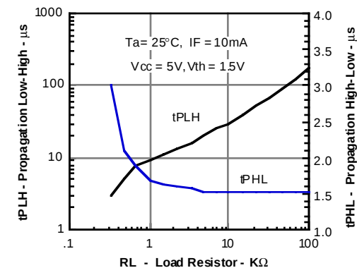
Figure 17. -1 Propagation delay versus collector load resistor
