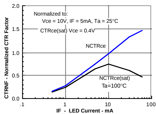
Figure 14. Normalization factor for non-saturated and saturated CTR T_A=85^{\circ}\text{C} versus I_F
