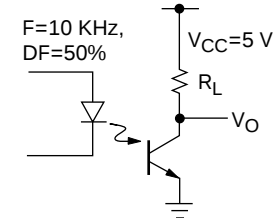
Figure 2. Saturated switching timing
