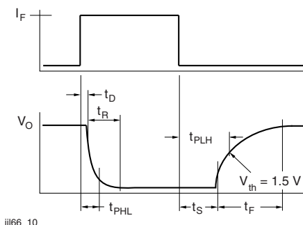
Fig. 10 - Switching Waveform
