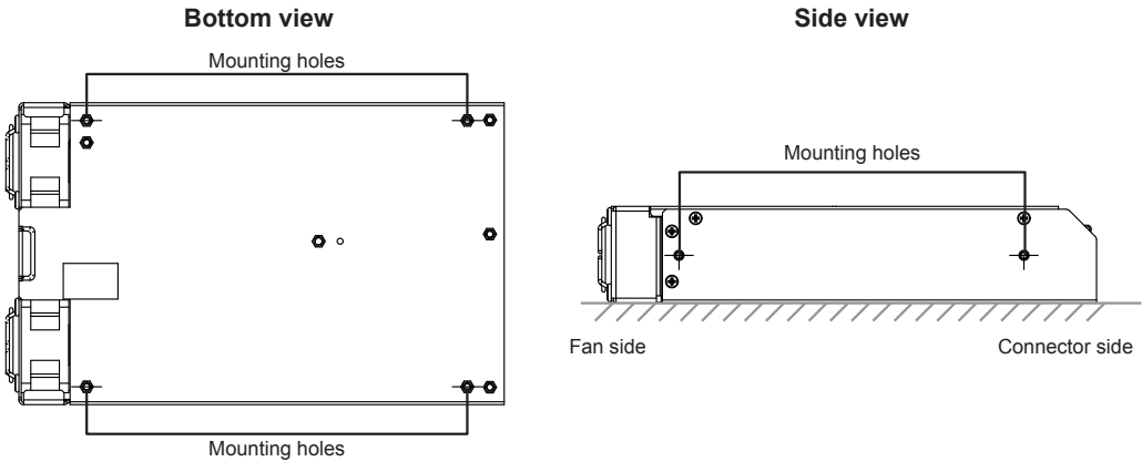
Fig. 5: Position of mounting holes
