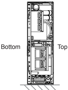
Fig. 4: Mounting on the right side
