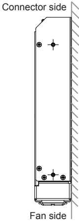
Fig. 2: Vertical mounting
