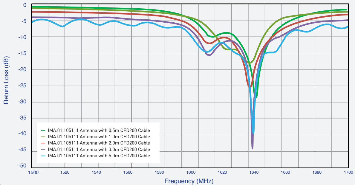
Figure 2. Return Loss of the IMA.01 antenna
