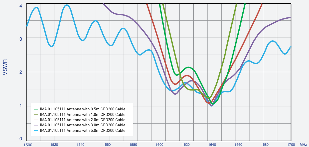
Figure 3. VSWR of the IMA.01 antenna.
