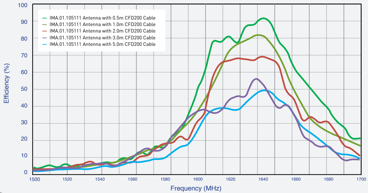
Figure 4. Efficiency of the IMA.01 antenna
