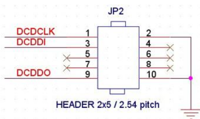
<Figure 3.3> W7100A Debugger Connector
