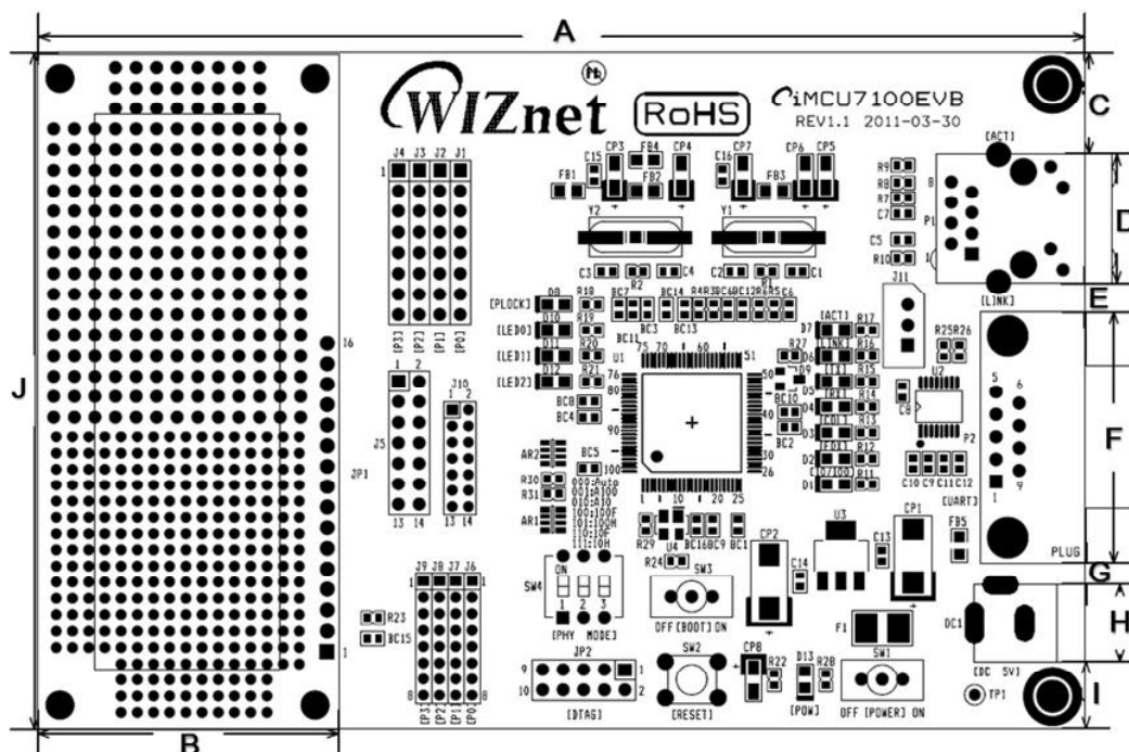
<Figure 3.5> iMCU7100EVB Dimension
