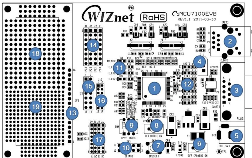
<Fig 3.1> Layout of iMCU7100EVB
