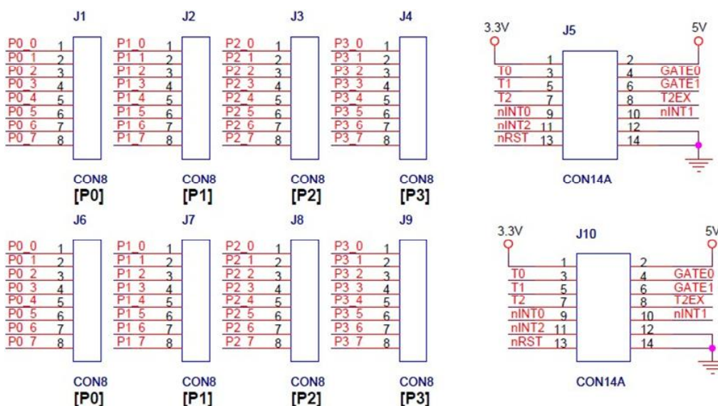
<Figure 3.4> Port Expansion Connector
