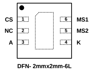
DFN- 2mmx2mm-6L
