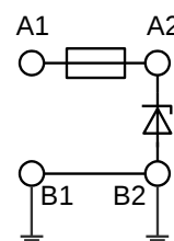
Fig 43. IP4389CX4 schematic view
