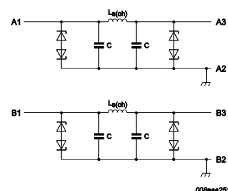
Fig 27. IP3047CX6 Schematic view
