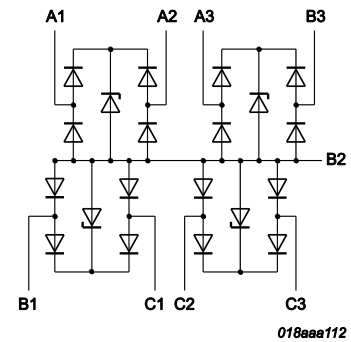
Fig 21. IP4309CX9 schematic view
