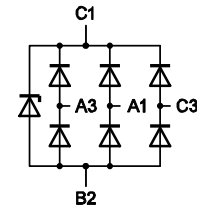
Fig 16. IP4059CX5 Schematic view and package drawing
