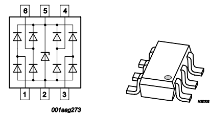
Fig 18. Schematic SC-74 package drawing
