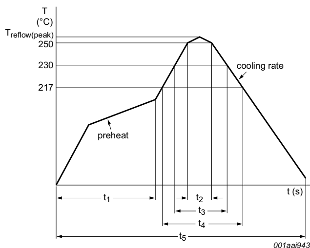
Fig 10. Pb-free solder reflow profile
