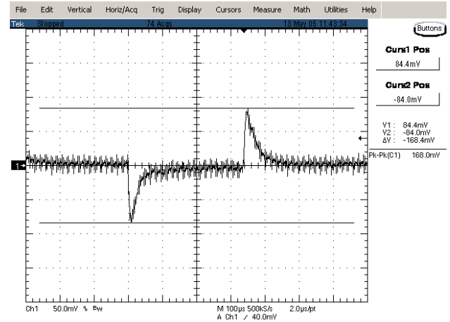
Figure 14: Typical transient response to step load change at 0.5A/\mu S from 50% to 100% of I_o , max at 36V in , 6.5V out (measurement with a 1μF ceramic)
