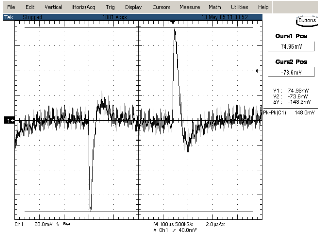
Figure 13: Typical transient response to step load change at 0.5A/\mu S from 100% to 50% of I_o , max at 24V in , 15.0V out (measurement with a 1μF ceramic)
