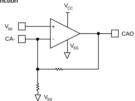
Figure 6. Diagnostic Feedback Operational Amplifier Circuit
