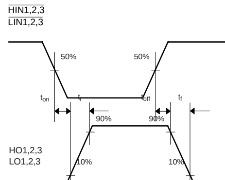
Figure 4. Input/Output Switching Time Waveform Definitions
