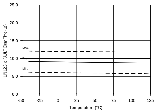
Figure 17A. \overline{\text{LIN1,2,3}} to \overline{\text{FAULT}} Clear Time vs. Temperature
