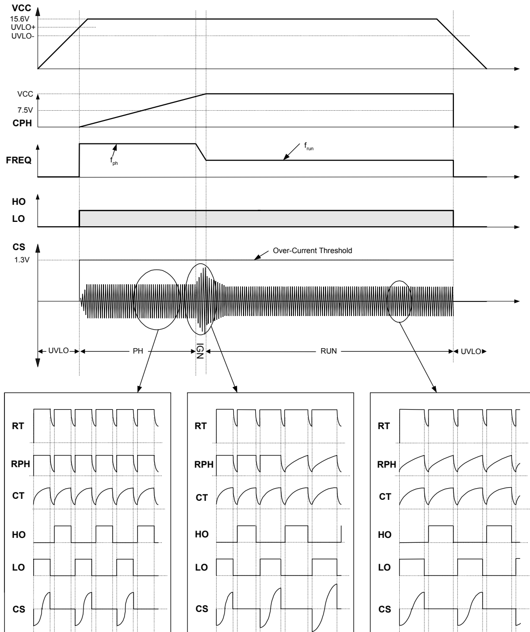
BALLAST TIMING DIAGRAMS NORMAL OPERATION
