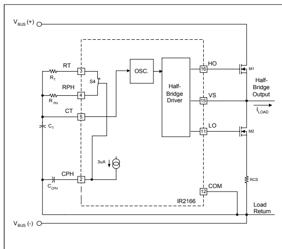
Figure 3, Preheat circuitry.
