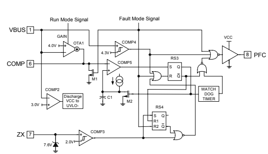
Figure 9: IR2166 detailed PFC control circuit
