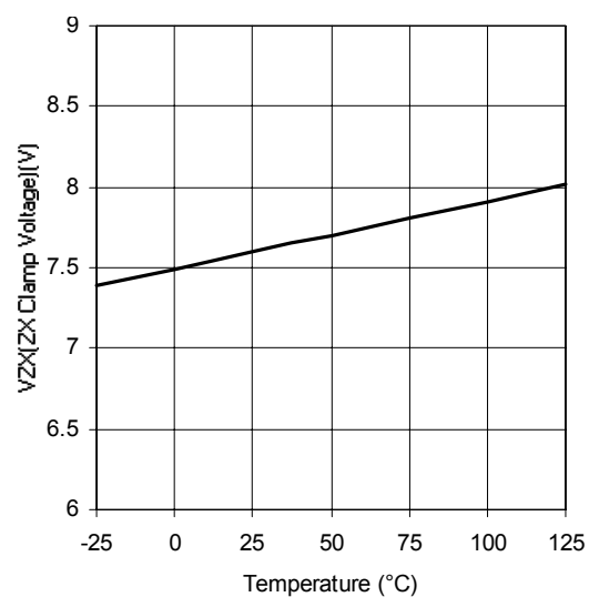
Graph 10: VZX (ZX Clamp Voltage) vs TEMP
