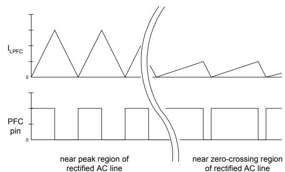
Figure 11: On-time modulation near the zero-crossings.
