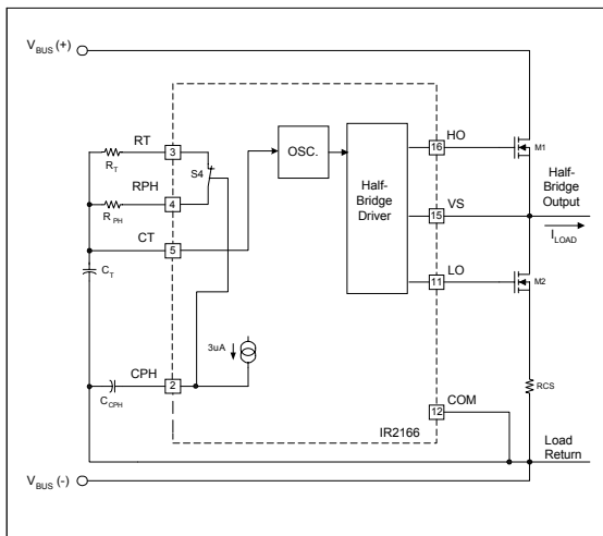
Figure 3, Preheat circuitry.
