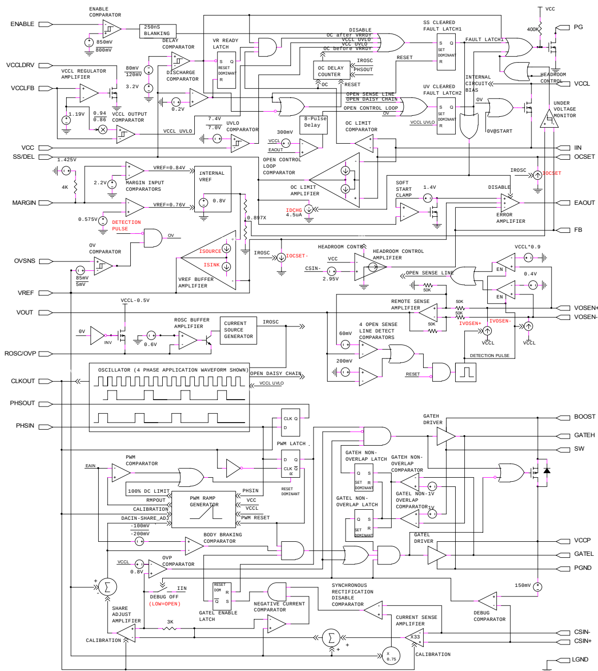
Figure 7 - Block Diagram
