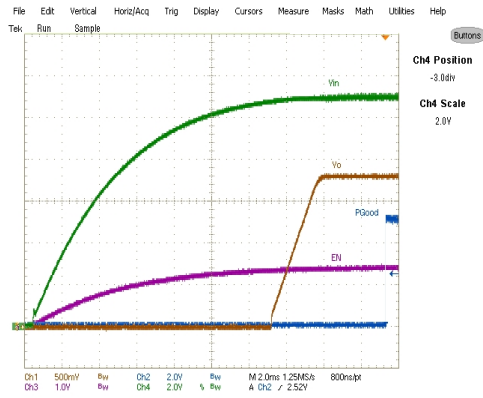
Fig. 22: Start up at 14A Load (Note 5) Ch 1 :V out Ch 2 :PGood Ch 3 :EN Ch 4 : V in
