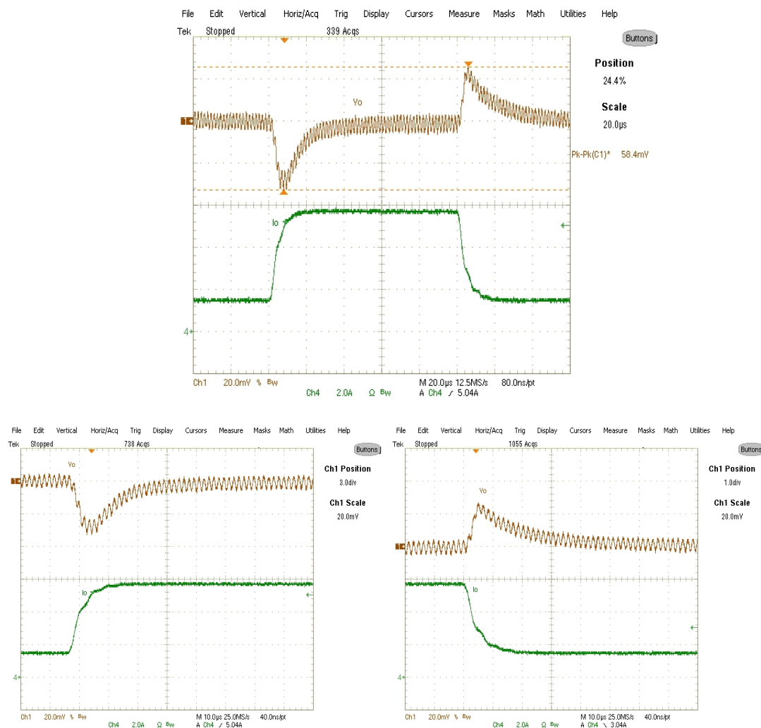
Fig. 28: Transient Response 1.4A(10%)-5.6A(40%) load (0.5A/μs) Ch_1:V_{out} , Ch_4:I_o
