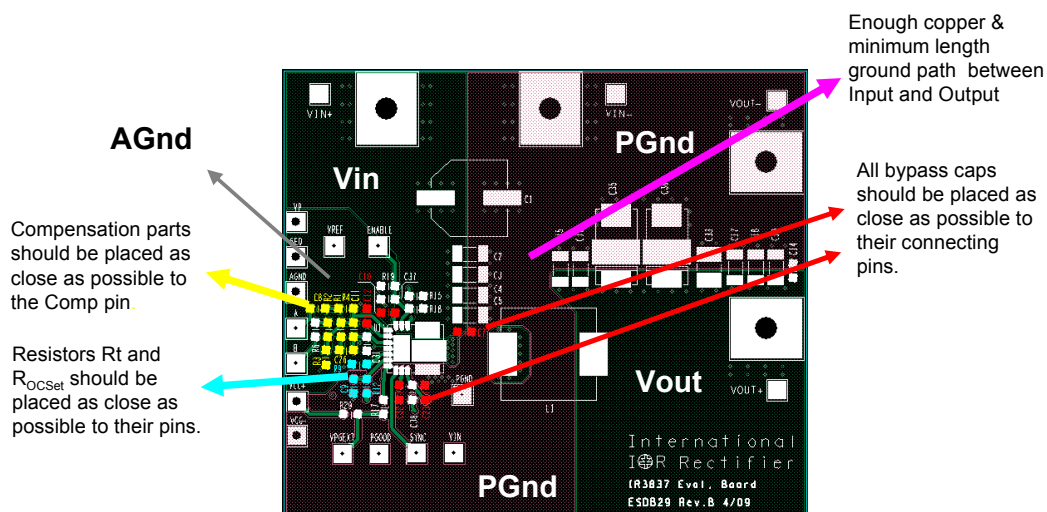
Fig. 30a. IRDC3837 Demoboard layout considerations – Top Layer
