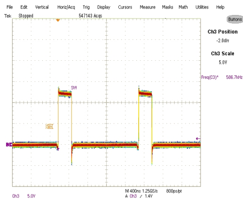
Fig. 26: Inductor node at 14A load Ch 3 :SW
