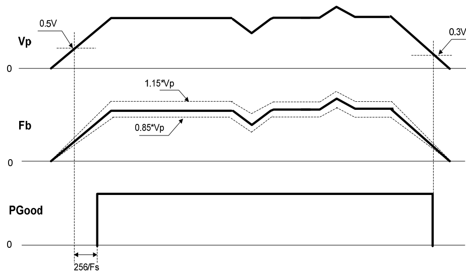
Fig.12 V_p Tracking ( V_{ref} > 1.5V , SS=H )
