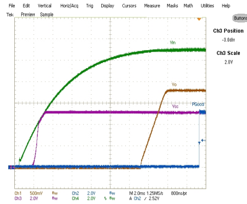
Fig. 23: Start up at 14A Load (Note 5) Ch 1 :V out Ch 2 :PGood Ch 3 :V cc Ch 4 : V in
