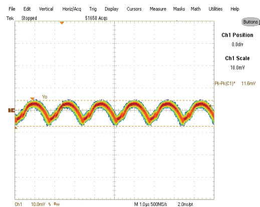
Fig. 25: Output Voltage Ripple, 10A load Ch1: V_{out}
