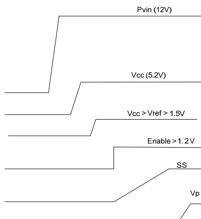
Fig. 4c. Recommended startup for memory tracking operation (Vtt-DDR)
