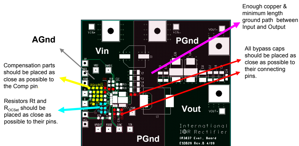
Fig. 30a. IRDC3838 Demoboard layout considerations – Top Layer
