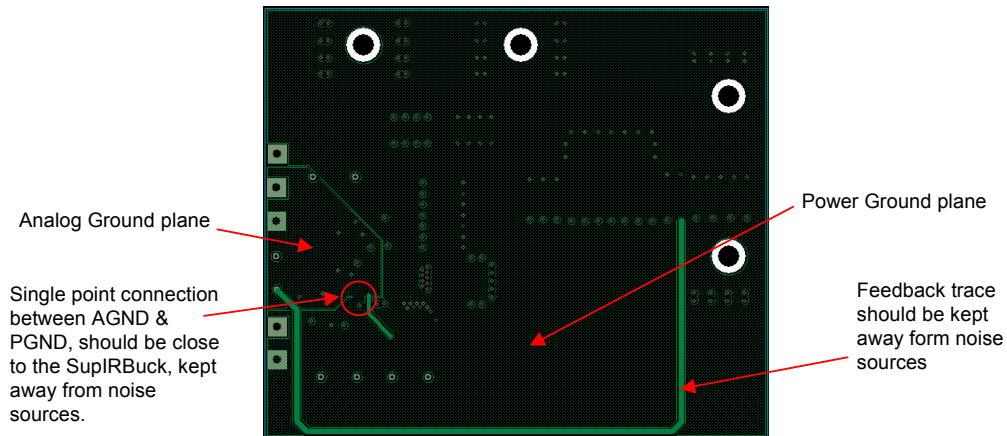
Fig. 30c. IRDC3838 demoboard layout considerations – Mid Layer 1
