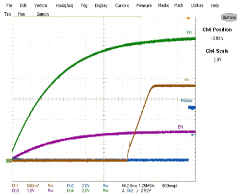
Fig. 22: Start up at 10A Load (Note 5) Ch 1 :V out Ch 2 :PGood Ch 3 :EN Ch 4 : V in
