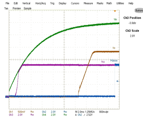
Fig. 23: Start up at 10A Load (Note 5) Ch 1 :V out Ch 2 :PGood Ch 3 :V cc Ch 4 : V in
