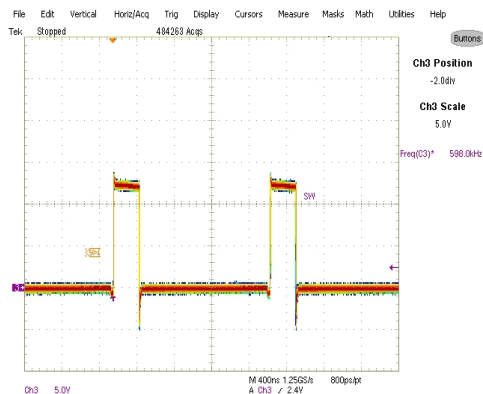
Fig. 26: Inductor node at 10A load Ch 3 :SW
