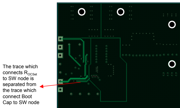
Fig. 30d. IRDC3838 demoboard layout considerations – Mid Layer 2
