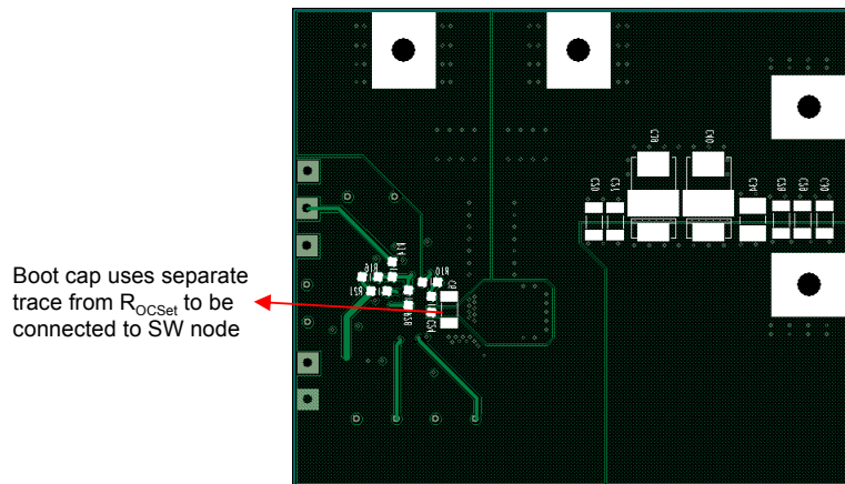
Fig. 30b. IRDC3838 demoboard layout considerations – Bottom Layer
