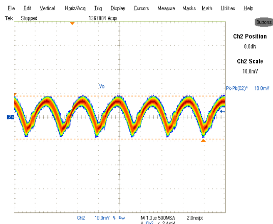
Fig. 20: Output Voltage Ripple, 14A load Ch 2 : V_{out}
