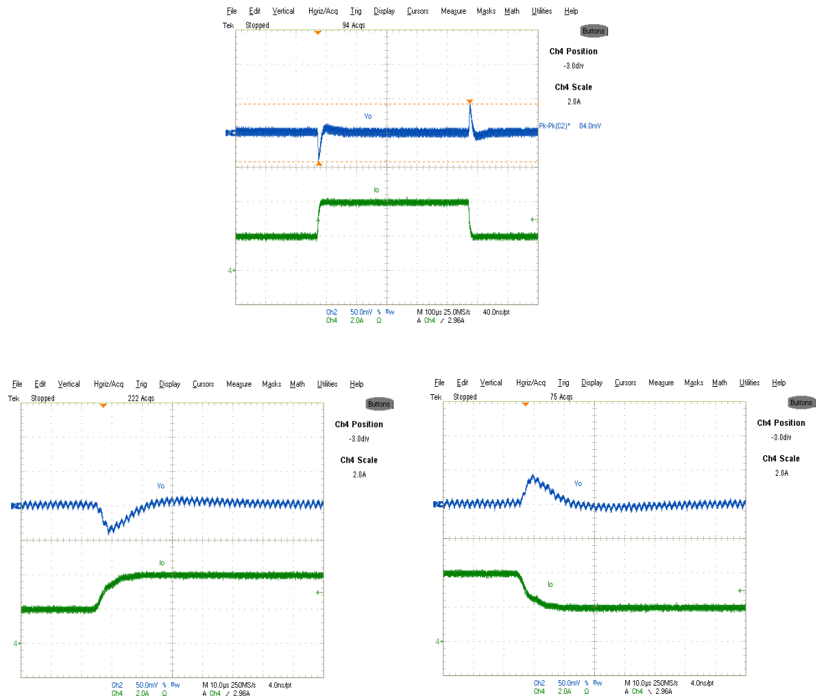
Fig. 23. Transient Response, 2A to 4A step 2.5A/μs Ch 2 :V o , Ch 4 :I o
