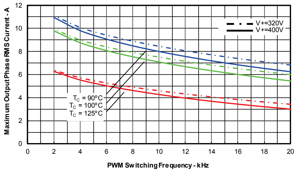
Figure 4. Maximum Sinusoidal Phase Current vs. PWM Switching Frequency Sinusoidal Modulation, T_J=150^{\circ}C , MI=0.8 , PF=0.6 , f_{mod}=50Hz
