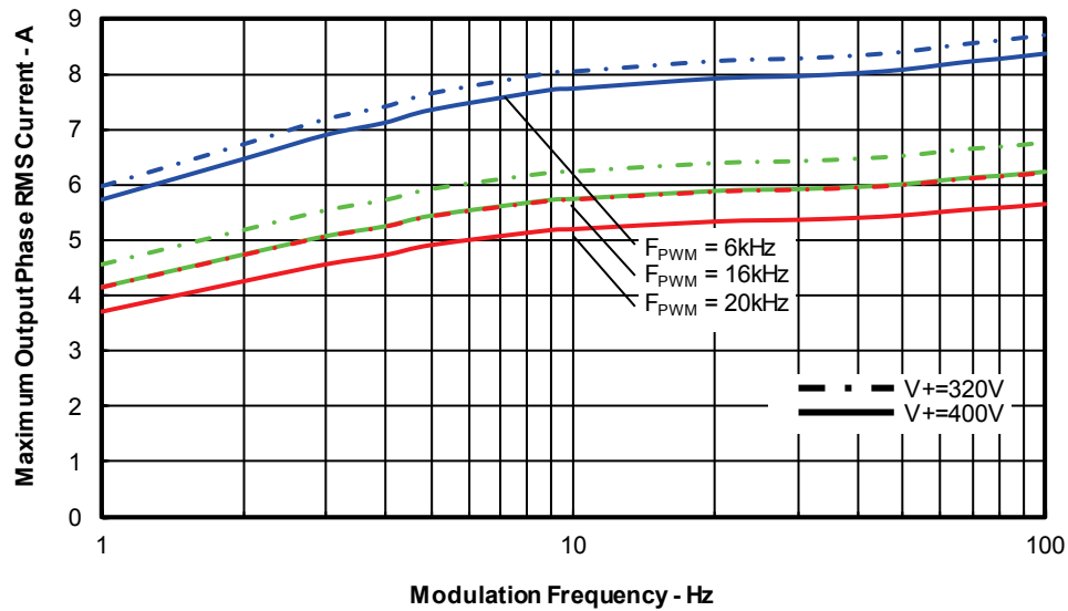
Figure 5. Maximum Sinusoidal Phase Current vs. Modulation Frequency Sinusoidal Modulation, T_J=150^{\circ}C , T_c=100^{\circ}C , MI=0.8 , PF=0.6
