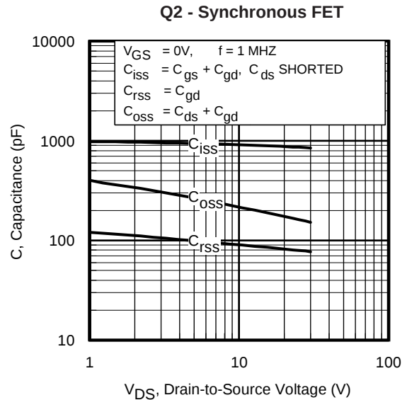
Fig 8. Typical Capacitance vs. Drain-to-Source Voltage
