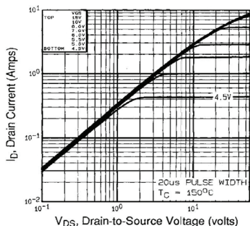
Fig. 2 - Typical Output Characteristics, T_C = 150^\circ\text{C}
