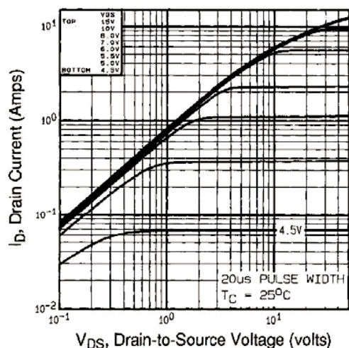
Fig. 1 - Typical Output Characteristics, T_C = 25^\circ C
