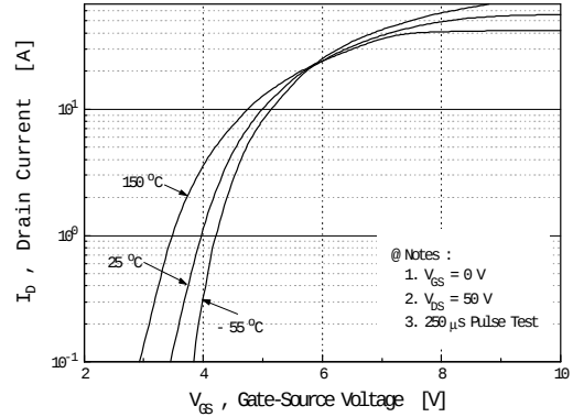
Fig 2. Transfer Characteristics
