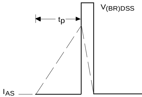
Fig 28b. Unclamped Inductive Waveforms
