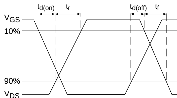
Fig 10b. Switching Time Waveforms
