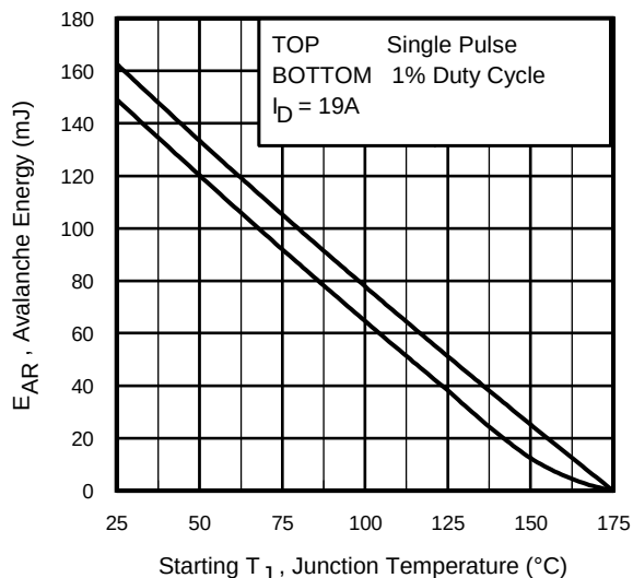
Fig 15. Maximum Avalanche Energy Vs. Temperature www.irf.com
