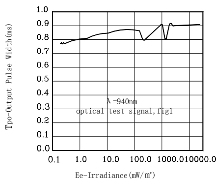
Figure1.Output Pulse Diagram
