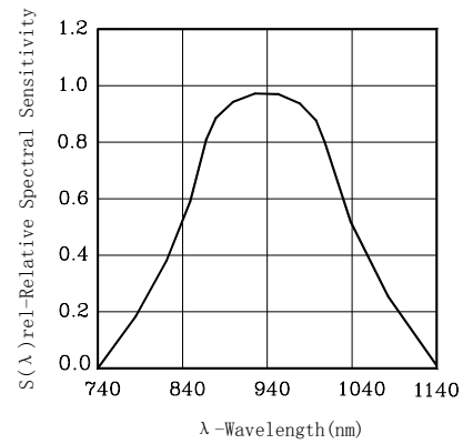
Figure9.Relative Spectral Sensitivity vs.wavelength
