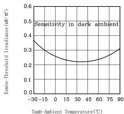
Figure8.Sensitivity vs.Ambient Temperature
