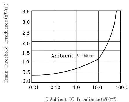
Figure4.Sensitivity In Bright Ambient
