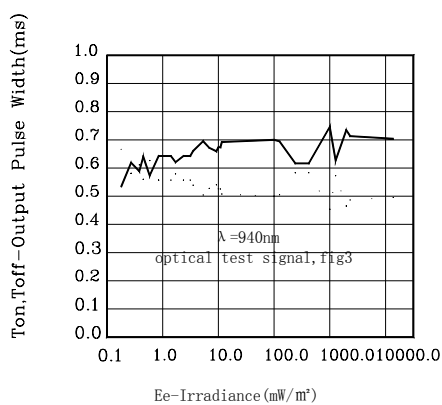
Figure2.Output Pulse Diagram
