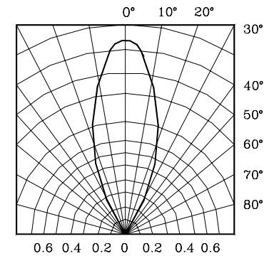
Figure10.Directivity
