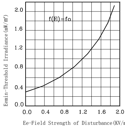
Figure6.Sensitivity vs.Electric Disturbances
