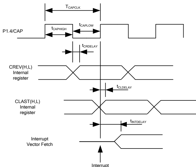
Figure 17. CAPTURE timing
