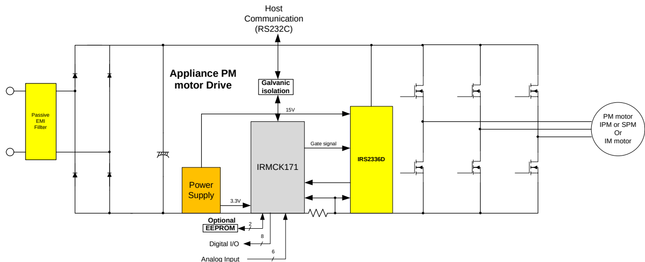
Figure 1 Typical Application Block Diagram Using IRMCK171
