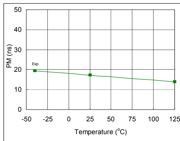
Fig. 67. Pulse Width Distortion vs. Temperature
