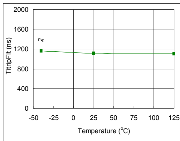
Fig. 69. ITRIP to Fault Time vs. Temperature
