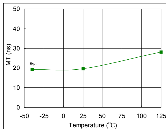
Fig. 65. Ton, Off Matching Time vs. Temperature
