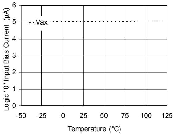
Figure 18A. Logic "0" Input Bias Current vs. Temperature
