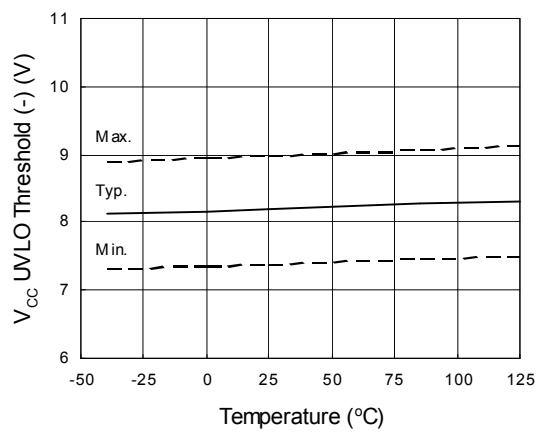
Figure 23. V CC Undervoltage Threshold (-) vs. Temperature
