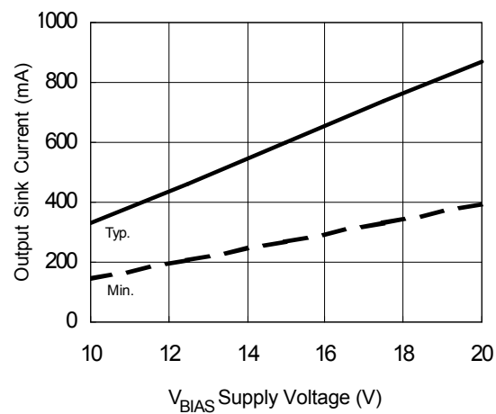
Figure 27B. Output Sink Currentt vs. Supply Voltage
