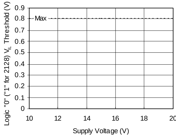
Figure 14B. Logic "0" ("1" for 2128) V_{IL} Threshold vs. Voltage
