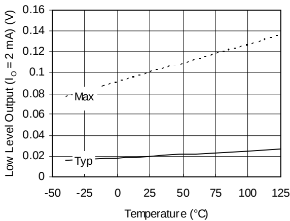
Figure 17A. Low Level Output ( I_o = 2 mA) vs. Temperature
