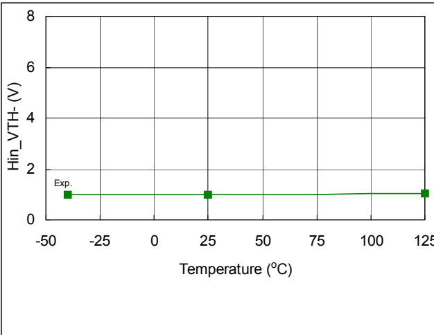
Fig. 50. Hin_VTH- vs. Temperature
