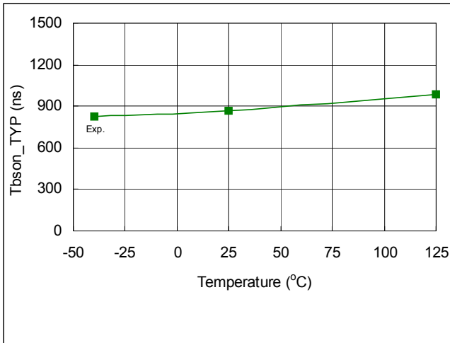
Fig. 35. Tbsn_TYP vs. Temperature
