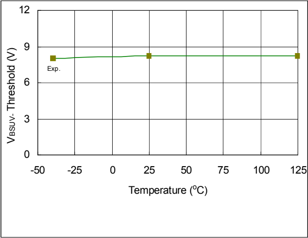
Fig. 46. V_{BSUV} Threshold vs. Temperature
