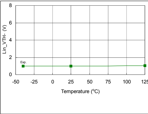
Fig. 48. Lin_VTH- vs. Temperature
