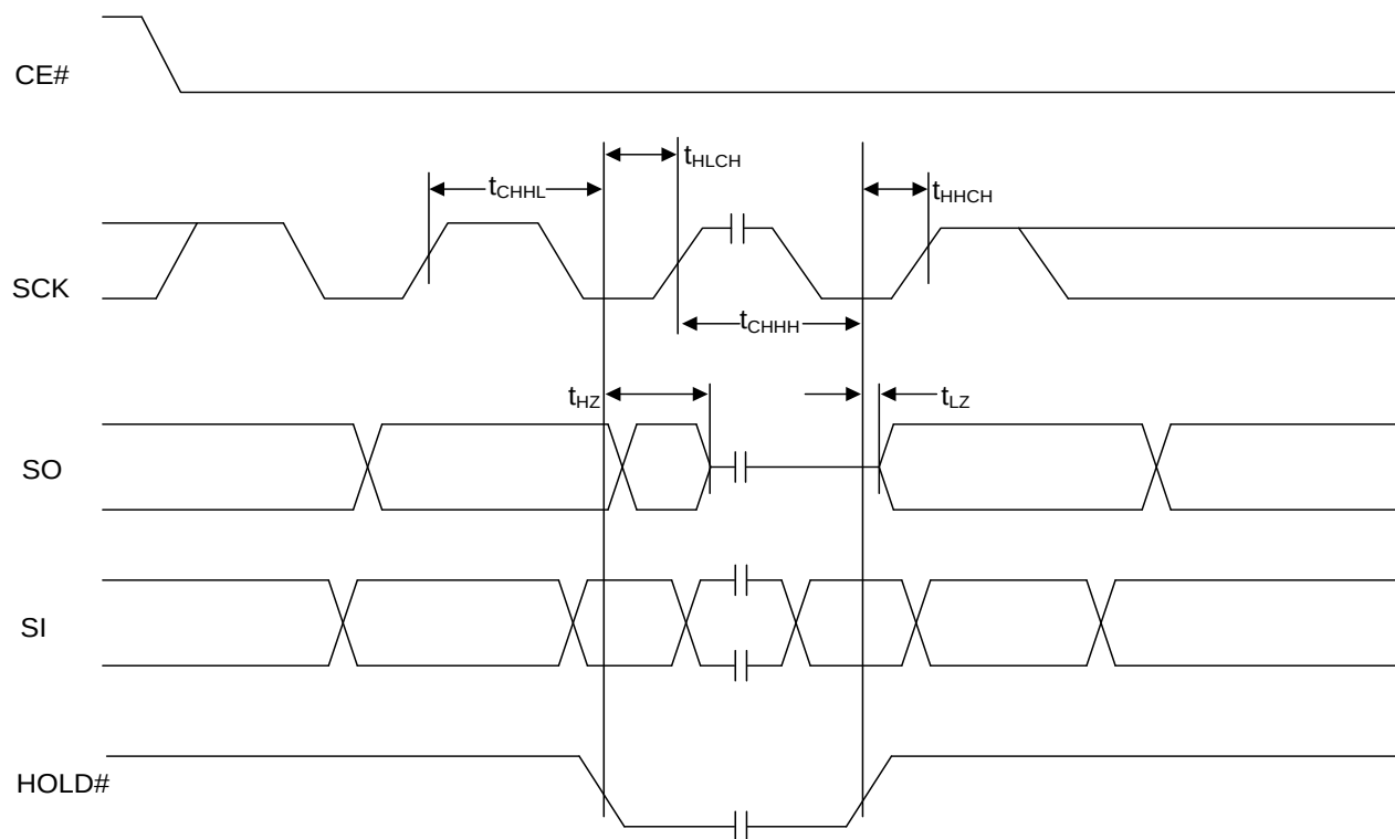
Figure 9.3 HOLD TIMING
