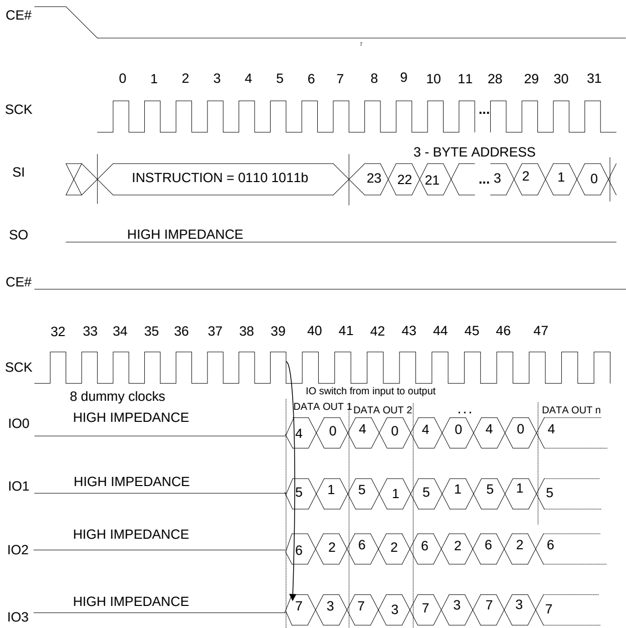
Figure 17. Fast Read Quad-Out Sequence
