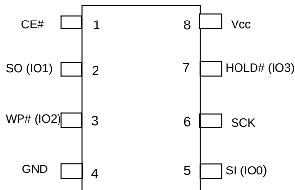
8-Pin SOIC
