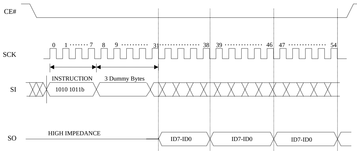
Figure 3. Read Product Identification Sequence: Command ABh
