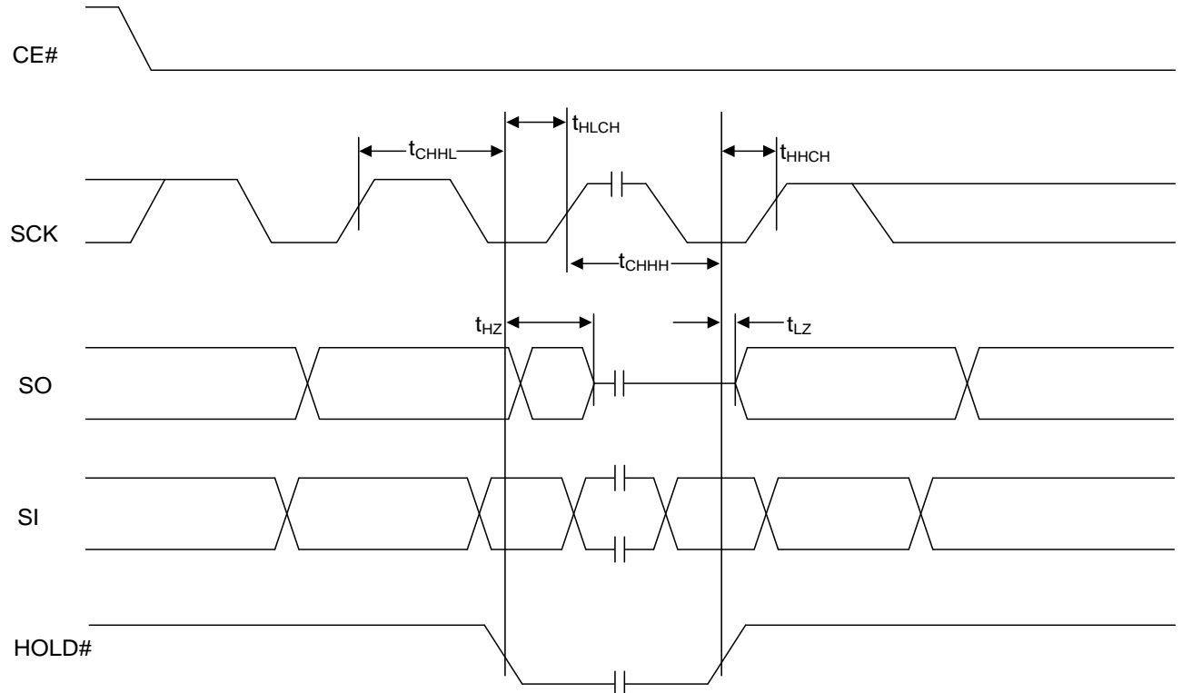
Figure 9.3 HOLD TIMING
