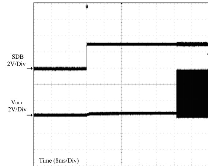
Figure 17 Turn On
