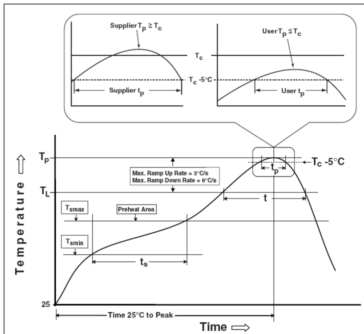
Figure 23 Classification Profile
